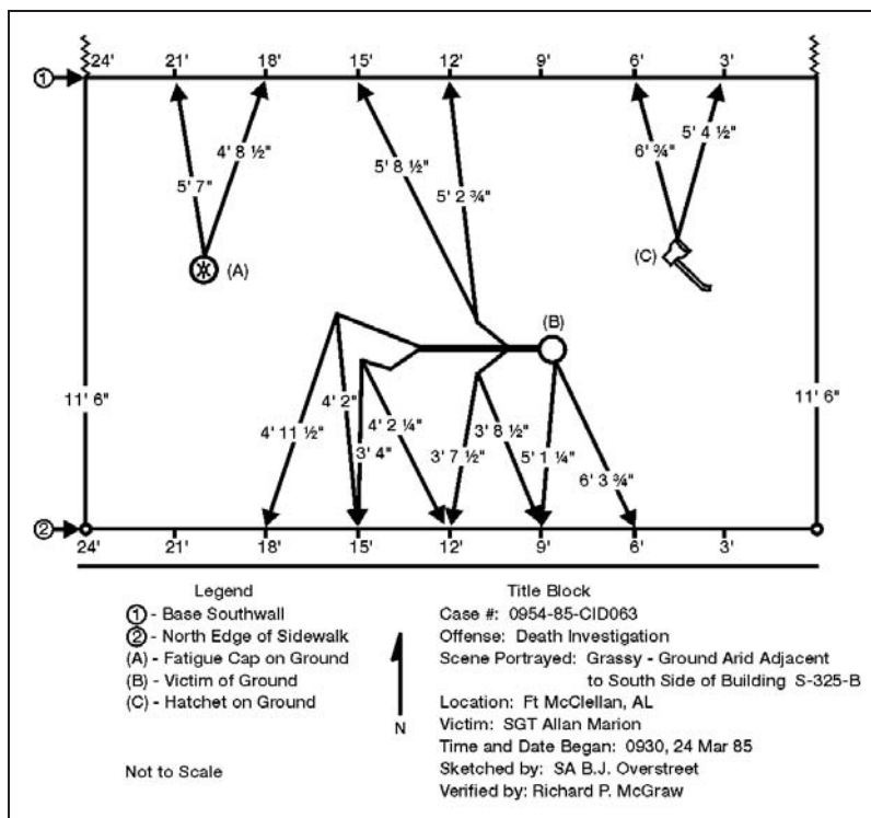
Figure 6-3. Triangulation Method
